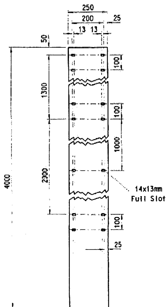
Item 1 - Backboard 250 x 50 Deal Board
